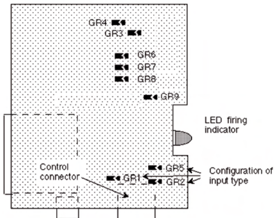
Positioning of 'Coffee beans' on board (solder-side view)
